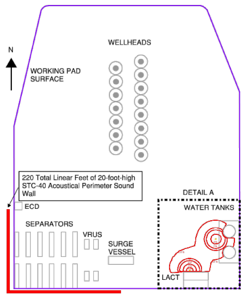
Production Pad Photometrics Scale 1" = 60'
