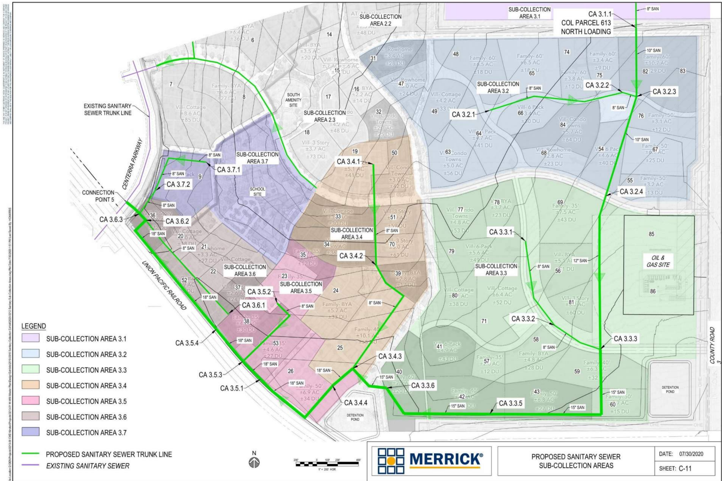
Figure 5.5 – Proposed Sanitary Sub-Collection Area 3
