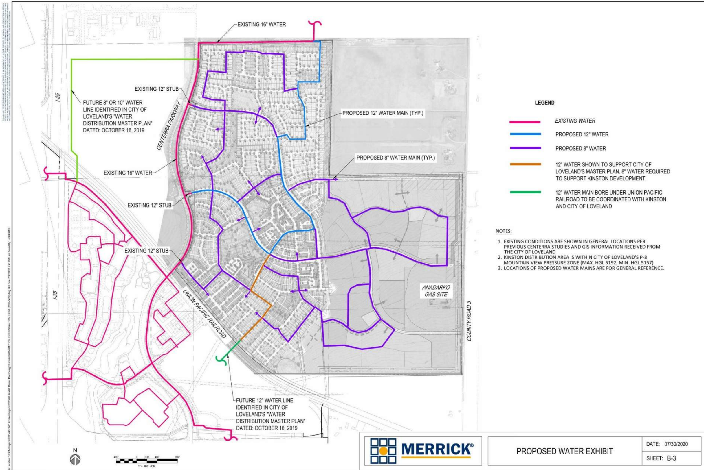
Figure 4.2 – Proposed Water Exhibit
