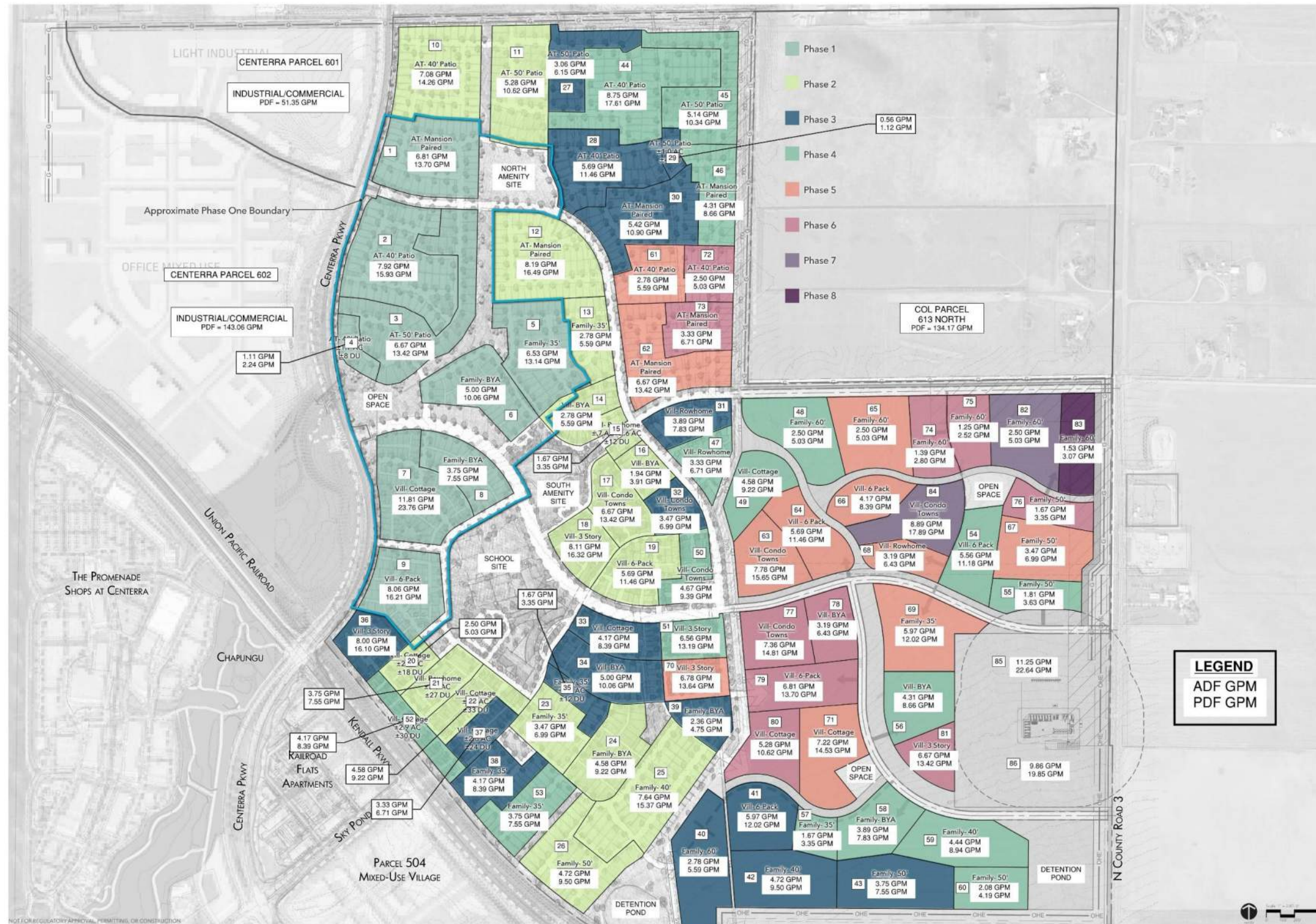
Figure 5.2 – Proposed Wastewater Loading Exhibit
